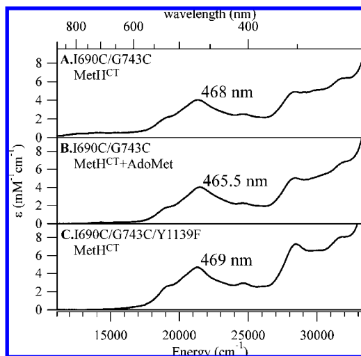
Figure 5. Abs spectra of (A) I690C/G743C MetH CT -bound Co 2+ Cbl, (B) I690C/G743C MetH CT -bound Co 2+ Cbl in the presence of excess AdoMet, and (C) I690C/G743C/Y1139F MetH CT -bound Co 2+ Cbl obtained at 310 K.
