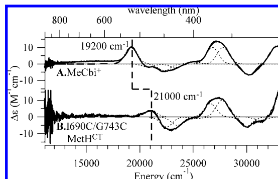
Figure 7. Solid lines: MCD spectra at 7 T of (A) aqueous MeCbl + and (B) I690C/G743C MetH CT -bound MeCbl obtained at 310 K. Dotted lines: Gaussian deconvolutions of the experimental spectra. Dashed lines: sum of individual Gaussian bands.
